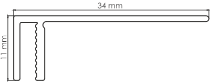
405 - Profile base 404
