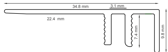
407 - Terminal (7&9mm)
