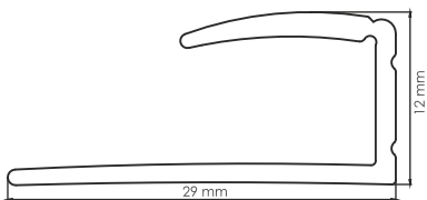
401 - Terminal (7mm)
