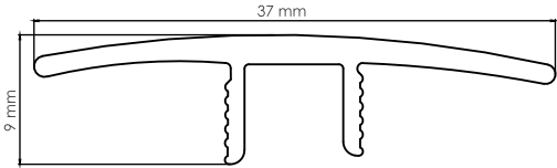
402 - Shrinkage - Expansion joint
