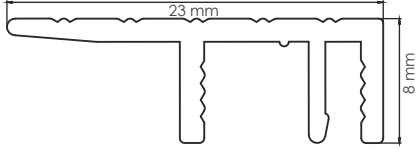
406 - Base for profiles 402, 403 & 407
