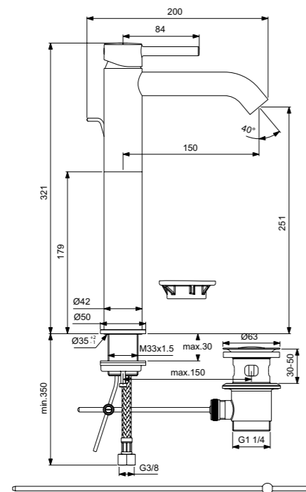
BC194AA
