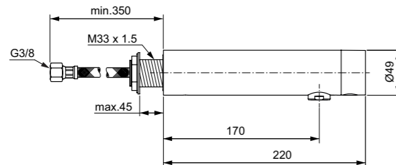
A7561AA
